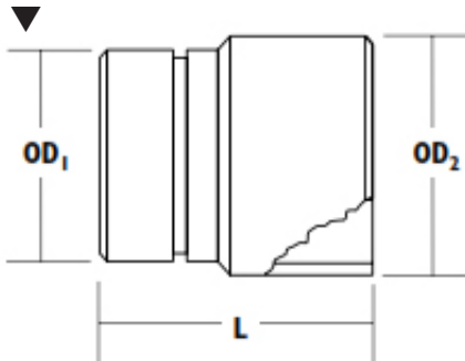
D2241 Certa-Lok® Yelomine® Solvent Weld IPS Adapters Certa-Lok® Male x IPS Solvent Weld Female
